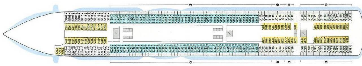
Deck 5
